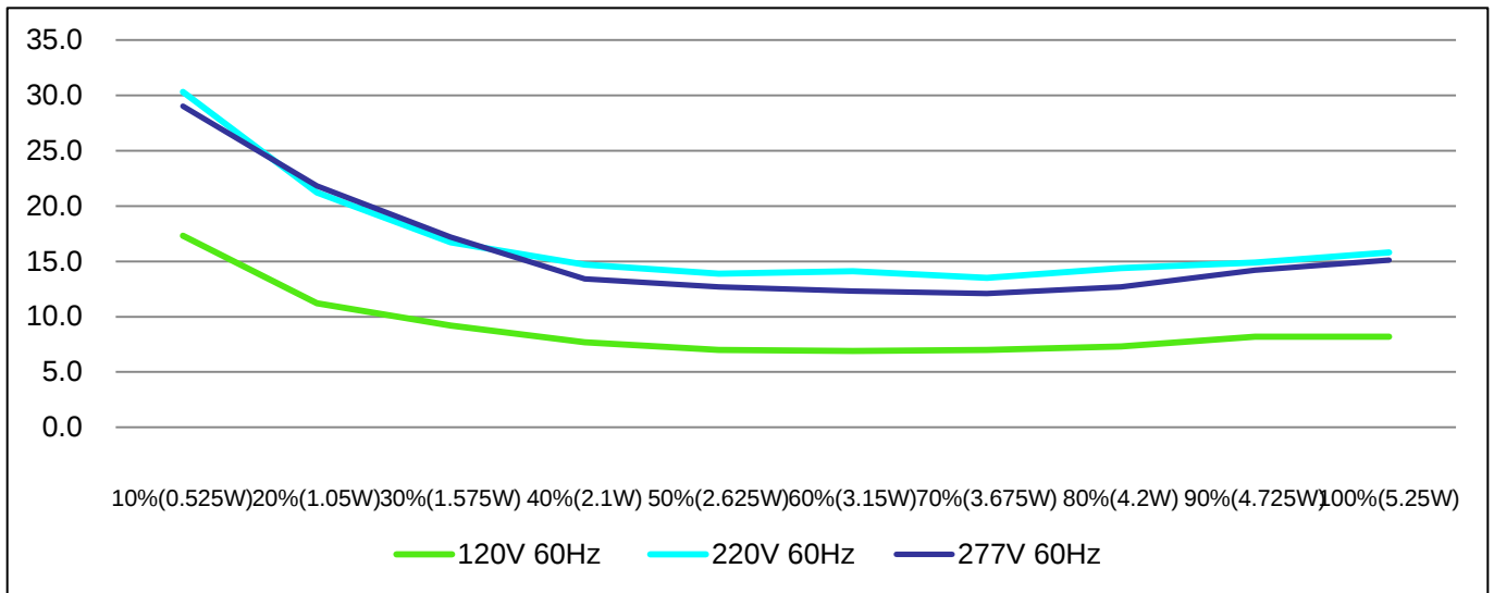
THD of the driver VS Power Output (W)
